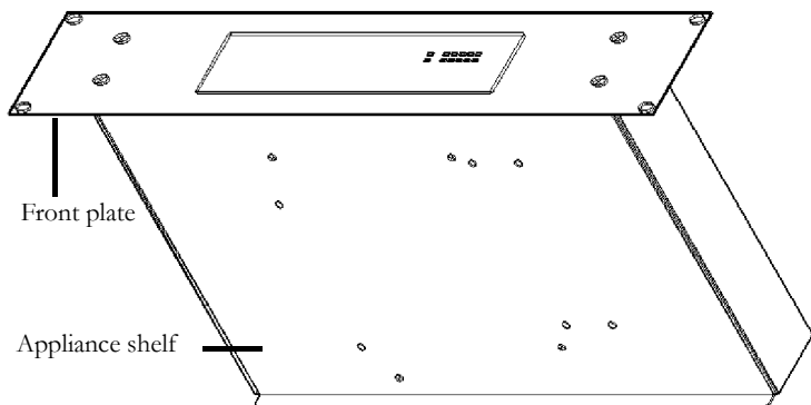
FIGURE 1 Assembled Rack-Mounting Kit Viewed from Front and Below
