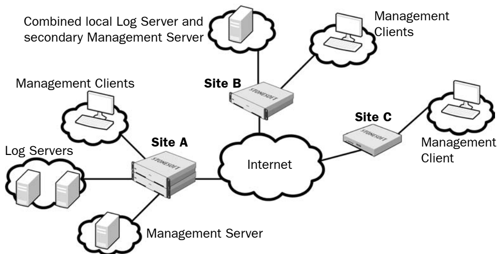
Illustration 3.1 Example of a Distributed Management Center Deployment
