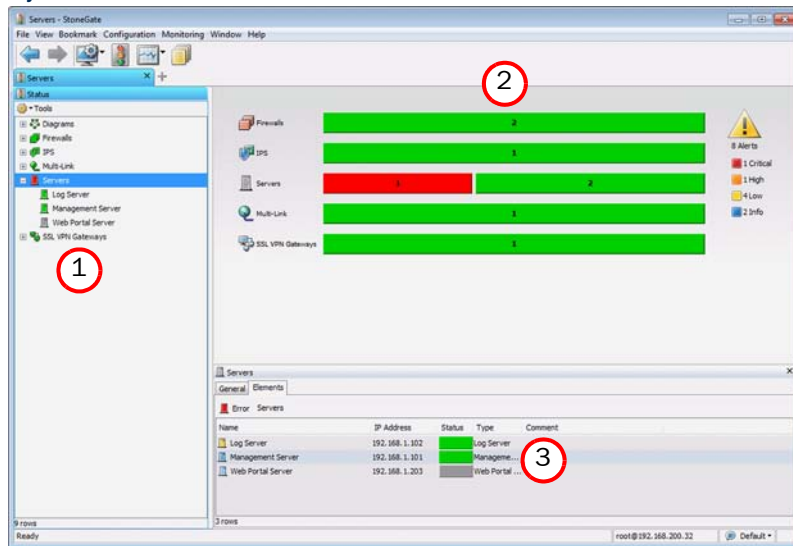
Illustration 4.2 System Status View
