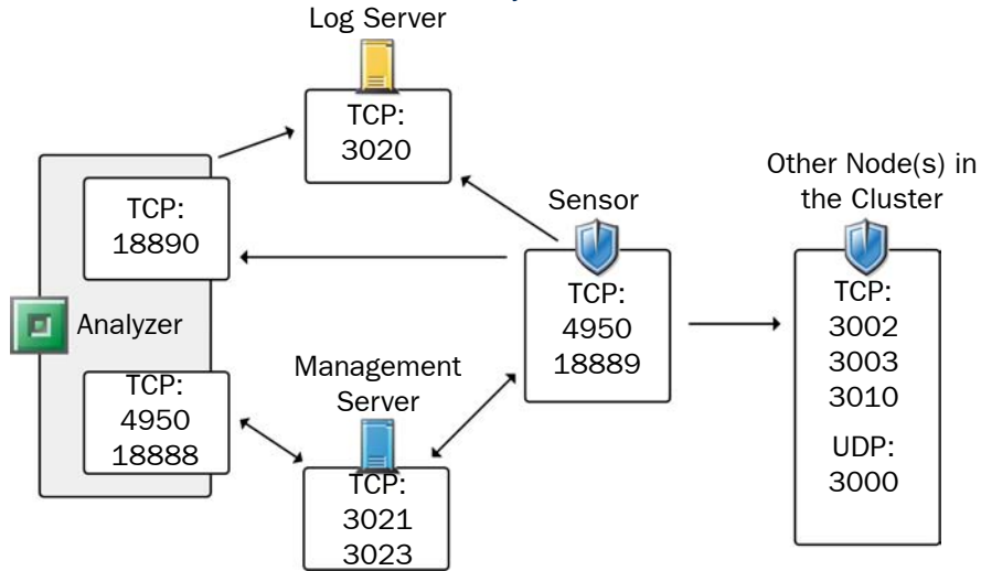
Illustration A.5 Default Destination Ports for Basic IPS System Communications
