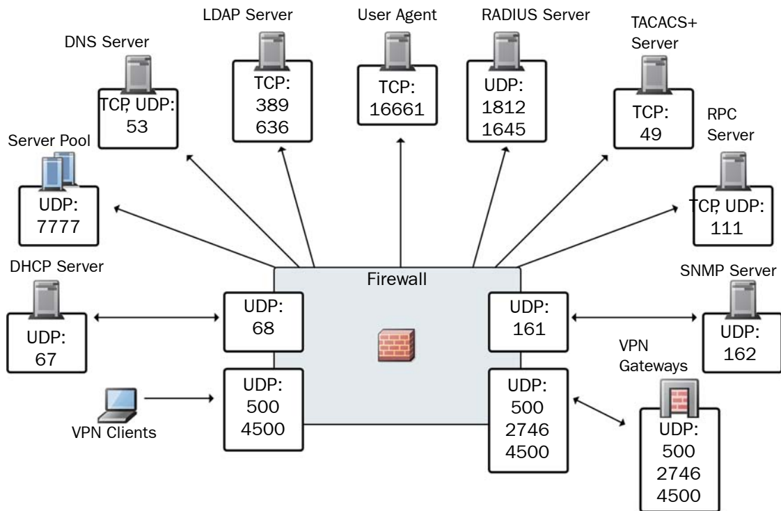
Illustration A.4 Default Destination Ports for Firewall/VPN Engine Service Communications
