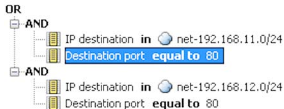
Illustration 10.1 Matching Events with a Filter
