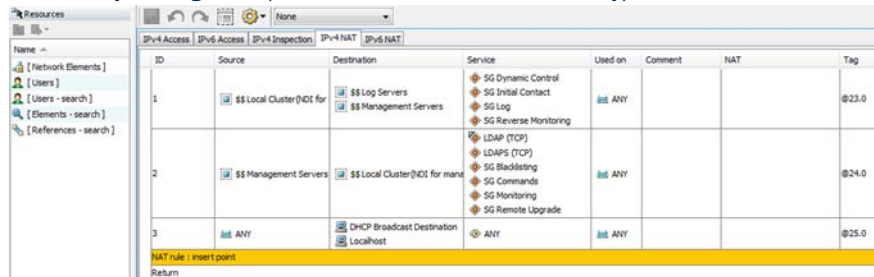
Illustration 4.10 Policy Editing View (IPv4 NAT rules in a Firewall Policy)
